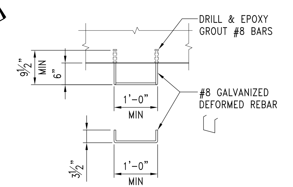
DETAIL SCALE: 3/4" = 1'-0" DROP RUNG STEP
