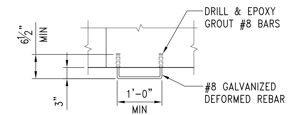
DETAIL SCALE: 3/4" = 1'-0" HANDHOLD
