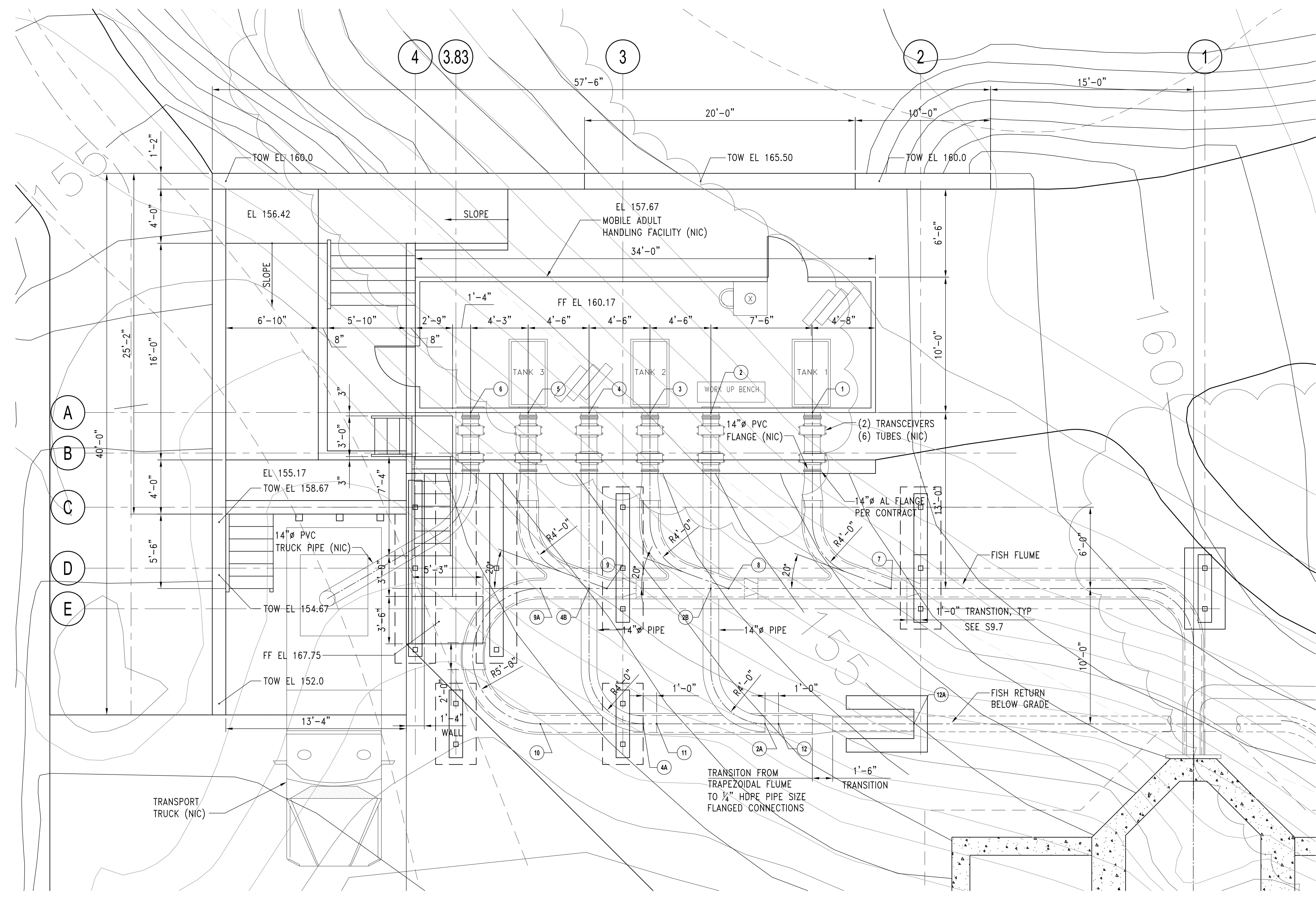
OVERALL PLAN ADULT CAPTURE AND SORTING FACILITY SCALE: 1/4" = 1'-0"
